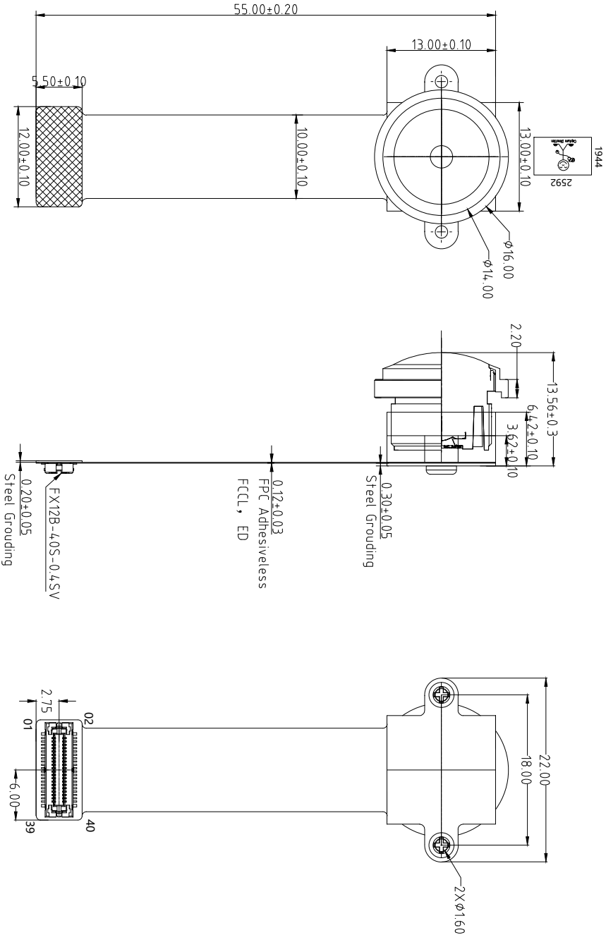
TOP VIEW
